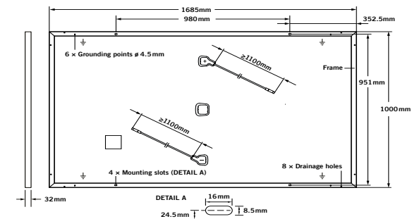
Fig. 1: External dimensions (in mm) and components for Q.PEAK DUO-G5.X, Q.PEAK DUO BLK-G5.X,
